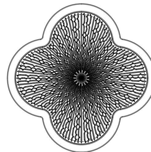
HANDLE DETAIL SCALE 1:1
